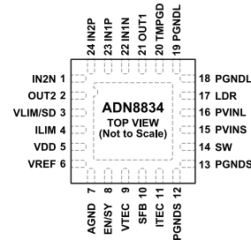
Figure 3. LFCSP Pin Configuration (Top View)
